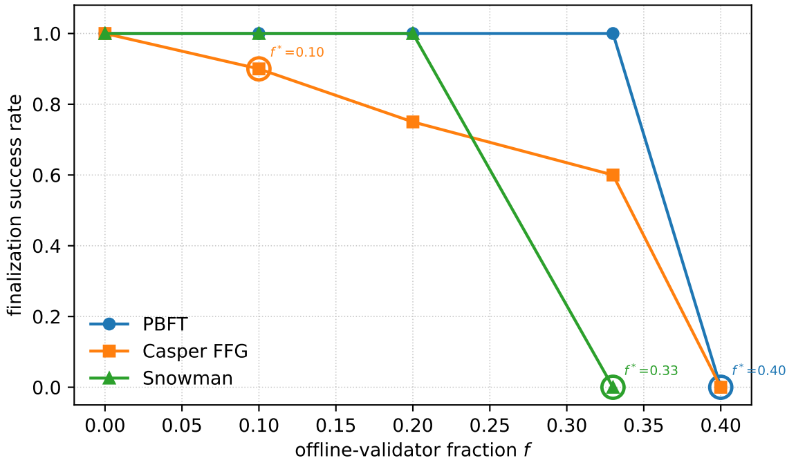
Finalization success vs offline fraction ( n = 25 , mean over 20 seeds)
