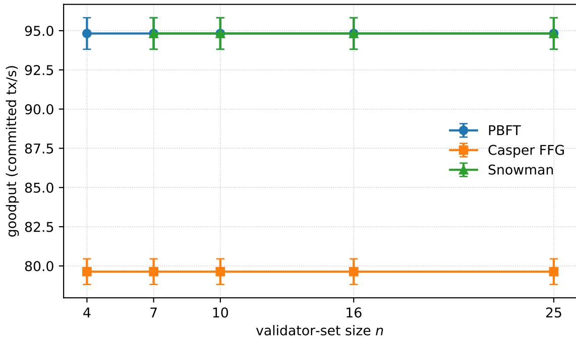
Goodput with 95% CI (workload-driven variance)
