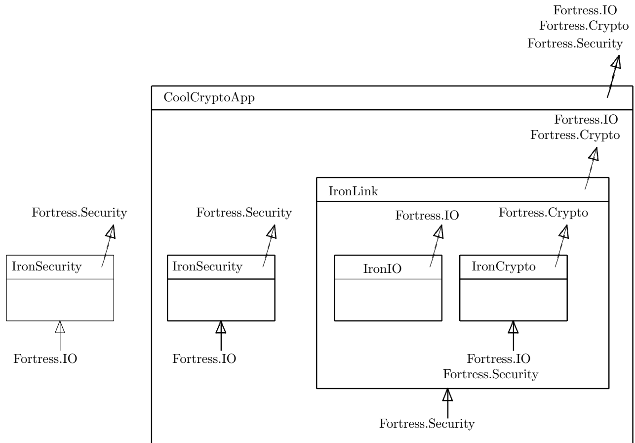
Figure 22.3: Repeated linking
