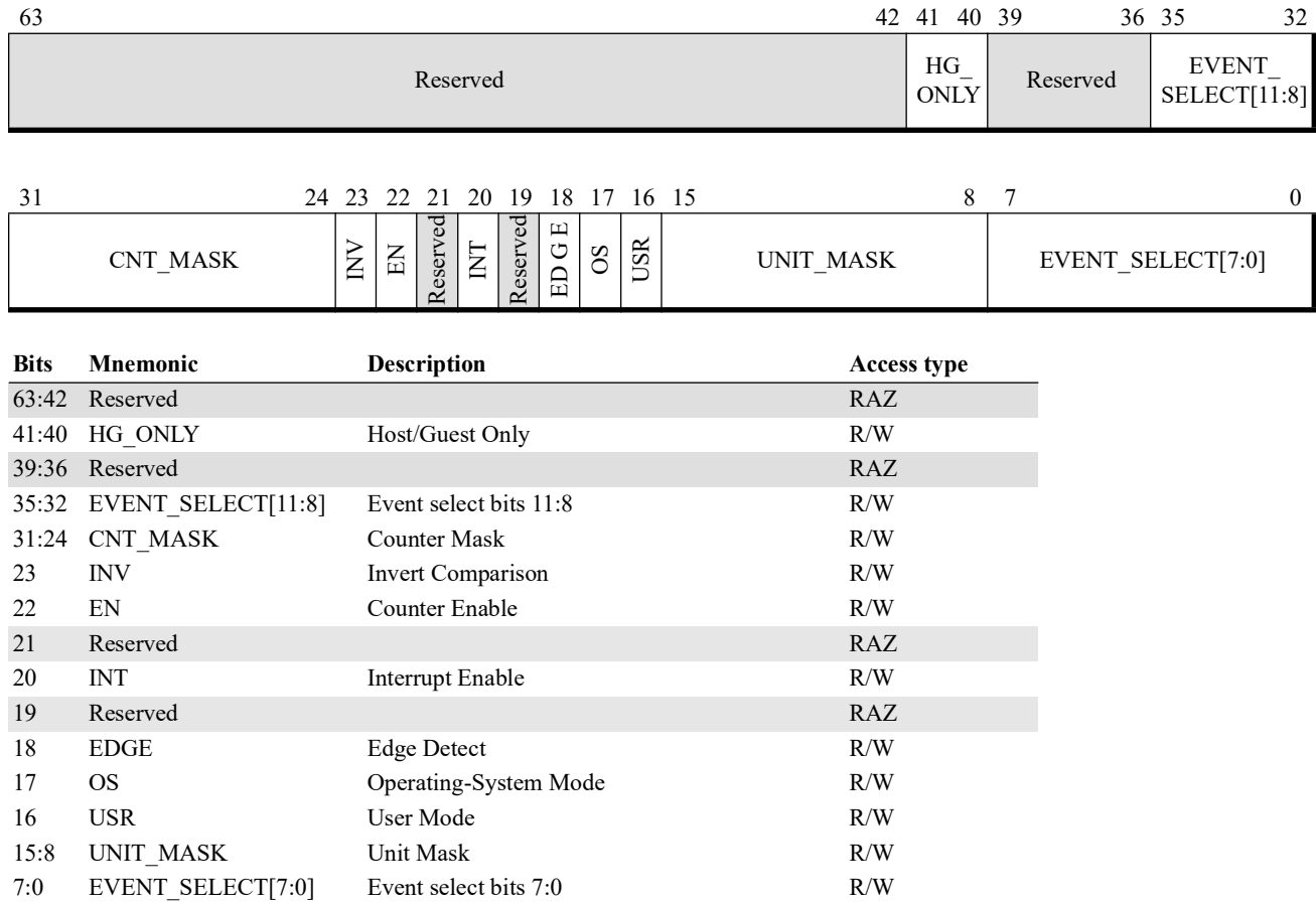
Figure 13-11. Core Performance Event-Select Register (PerfEvtSeln)
