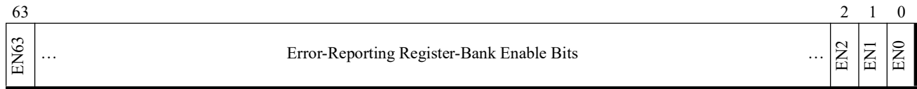
Figure 9-3. MCG_CTL Register
