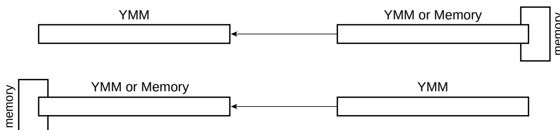
Figure 4-14. YMM Move Operations
