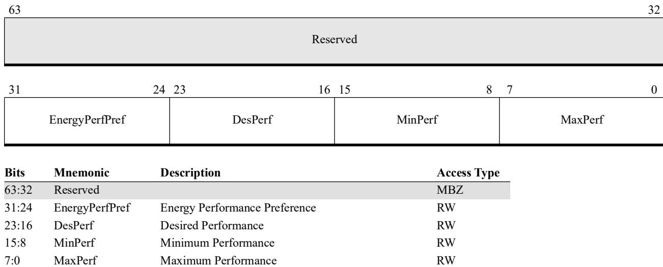
Figure 17-12. CPPC_REQUEST
