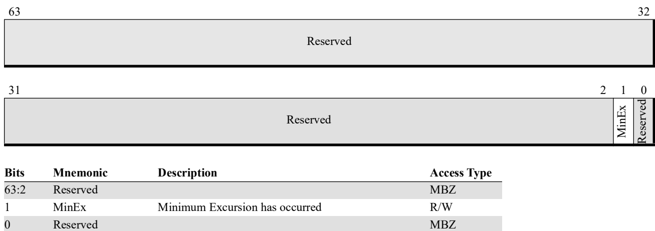
Figure 17-13. CPPC_STATUS
