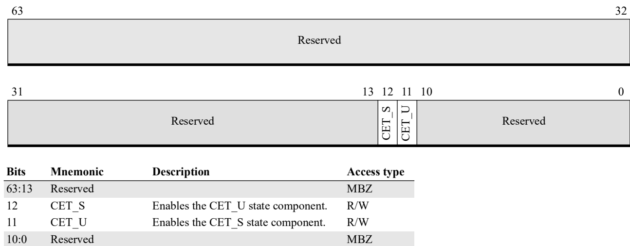
Figure 3-12. XSS Register
