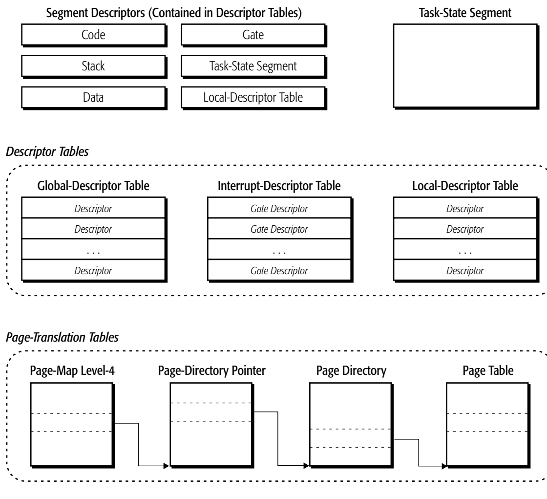
Figure 1-8. System-Data Structures
