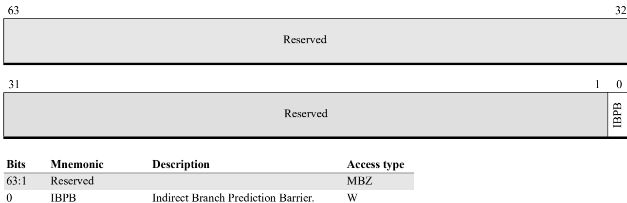
Figure 3-14. PRED_CMD Register (MSR 049h)
