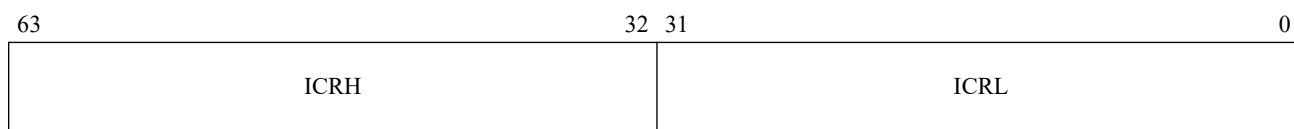
Figure 15-23. EXITINFO1
