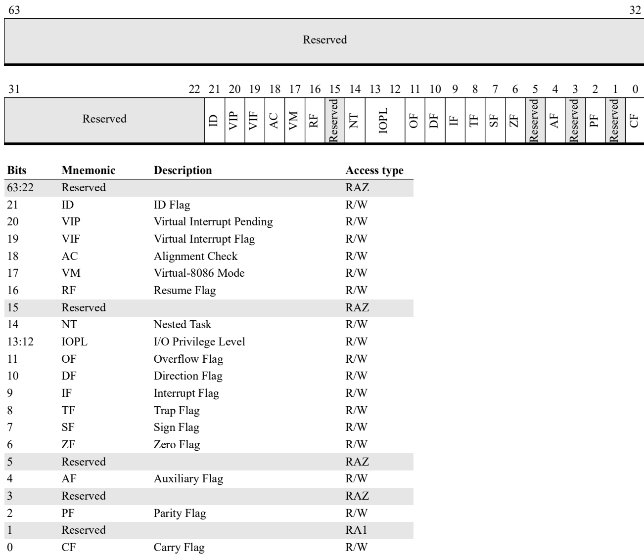
Figure 3-8. RFLAGS Register
