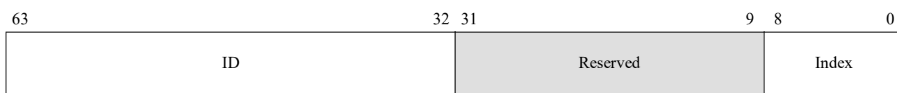
Figure 15-24. EXITINFO2
