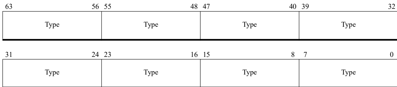
Figure 7-8. Fixed-Range MTRR
