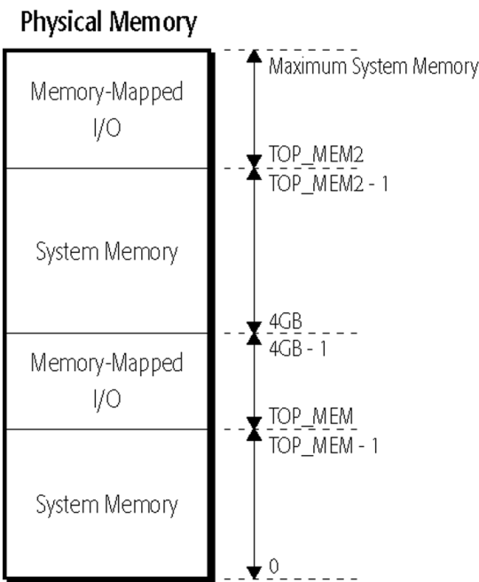
Figure 7-17. Memory Organization Using Top-of-Memory Registers
