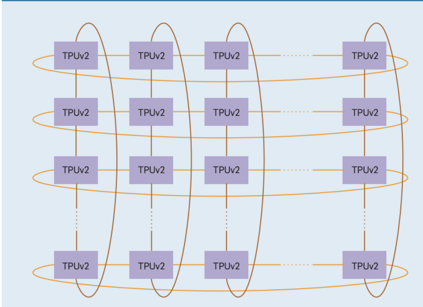
Figure 1. A 2D-torus topology. TPUv2 uses a 16x16 2D torus.
