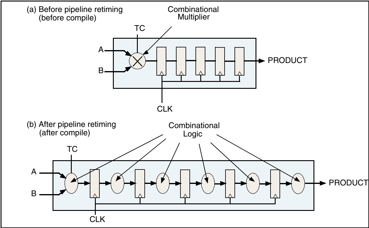
Figure 1-1 Block Diagram
