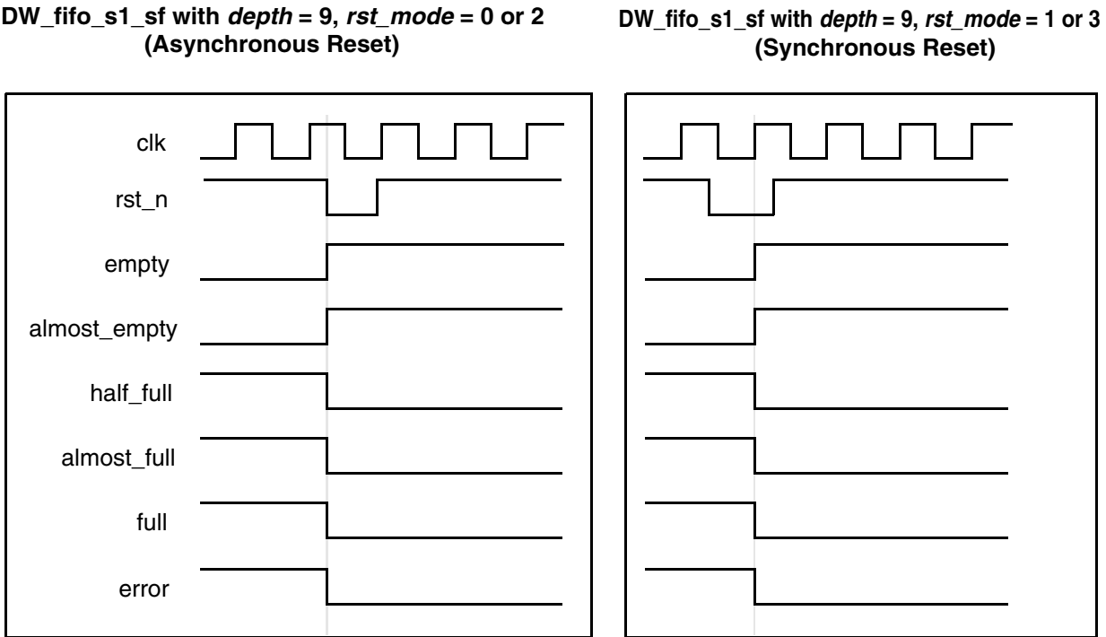
Figure 1-7 Reset Timing Waveforms
