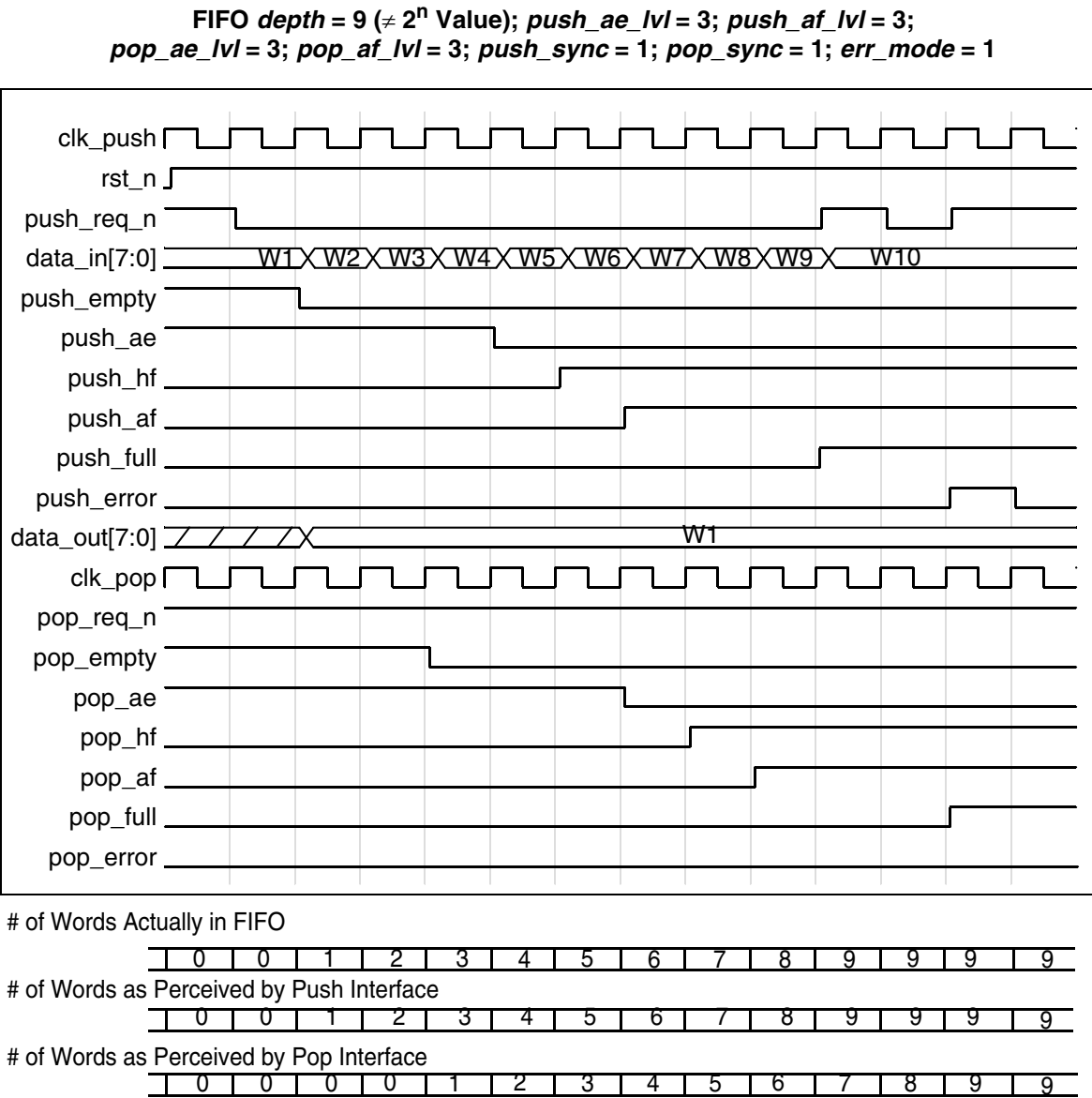
Figure 1-6 FIFO depth ≠ 2 n Push Timing Waveforms
