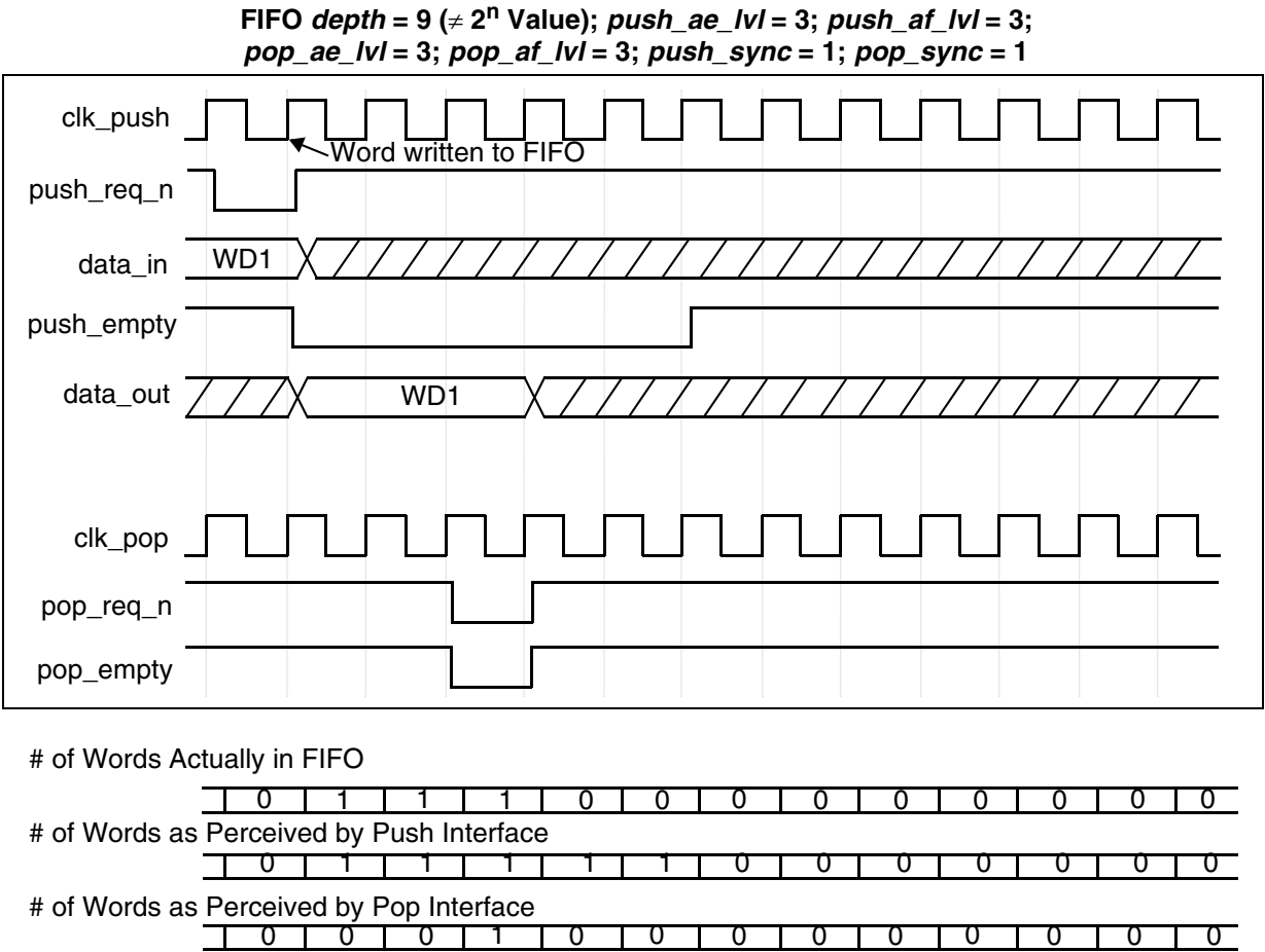
Figure 1-8 FIFO depth ≠ 2 n Single Word Timing Waveforms
