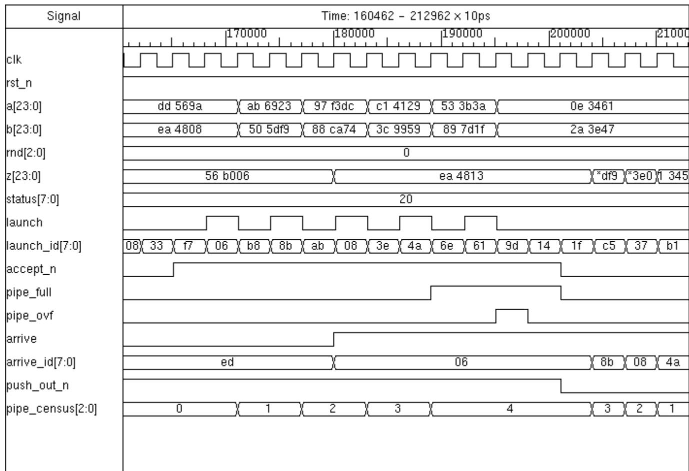
Figure 1-6 Push until Pipe Overflow Timing
