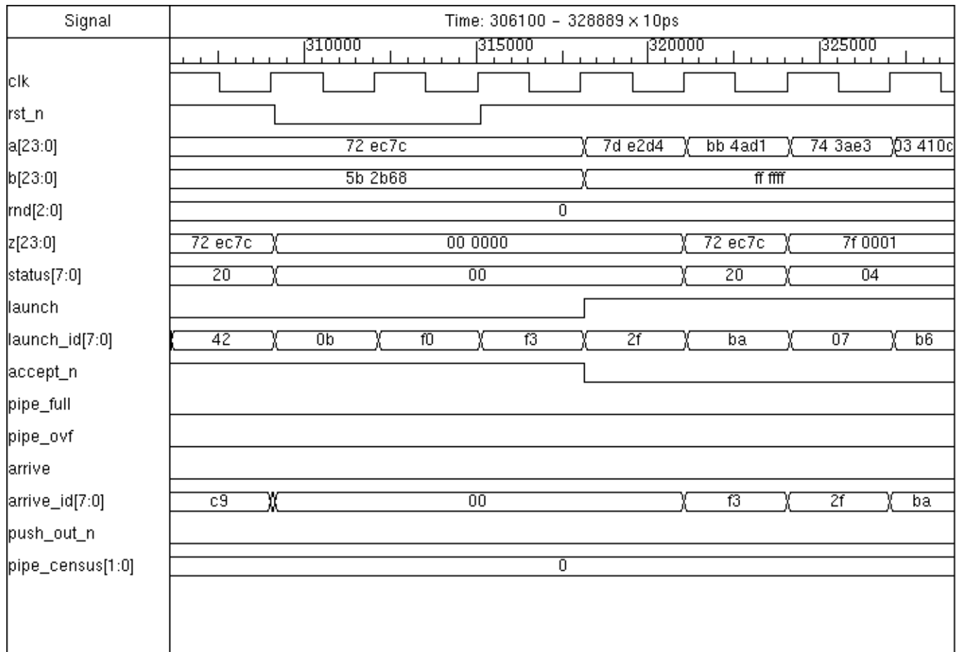
Figure 1-5 Asynchronous Reset Timing
