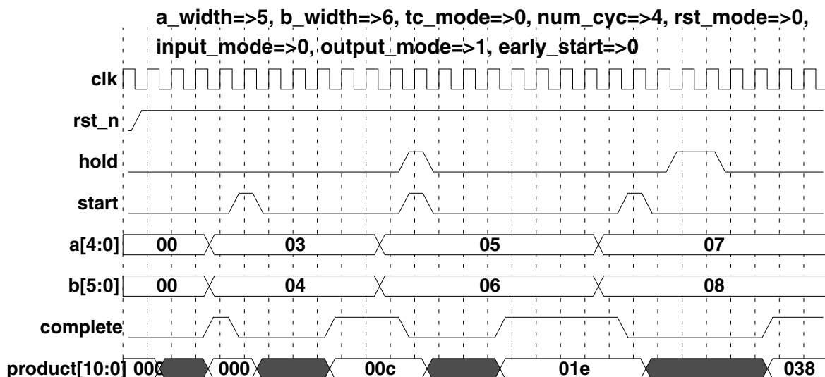
Figure 1-2 Simulation Waveform 2
