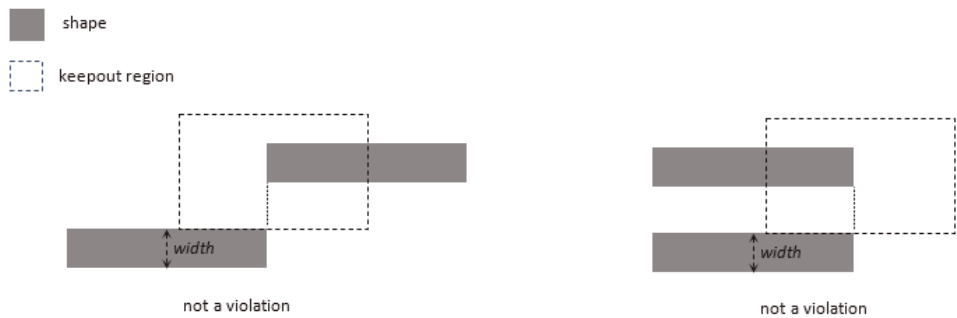
Figure 6 exceptAligned parameter set to 1 (all)
