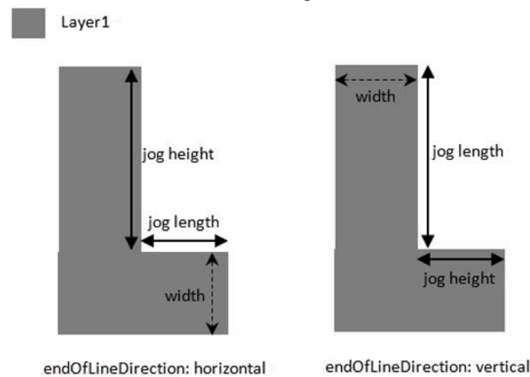
Figure 13 Minimum End Of Line Jog Distance Rule
