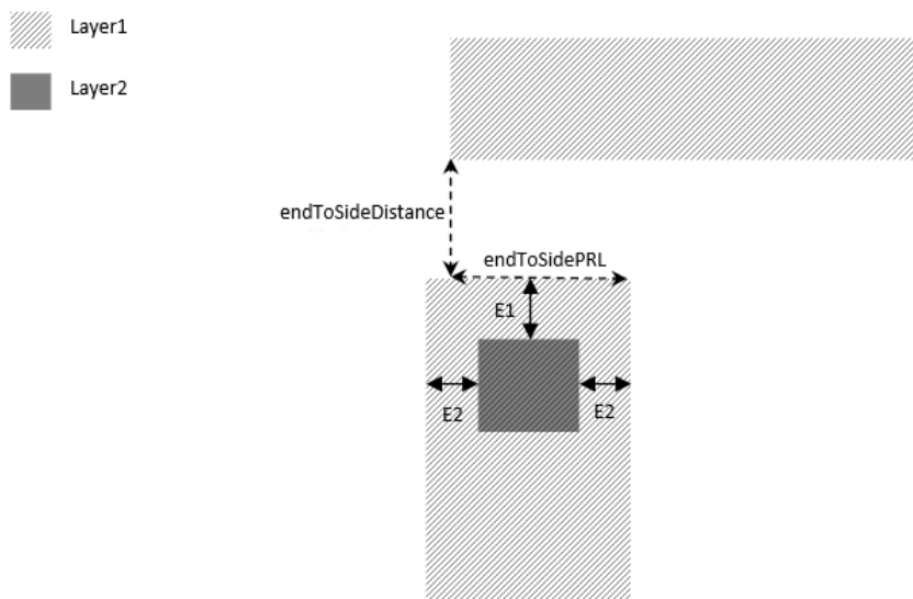
endToSideDistance and endToSidePRL parameters
