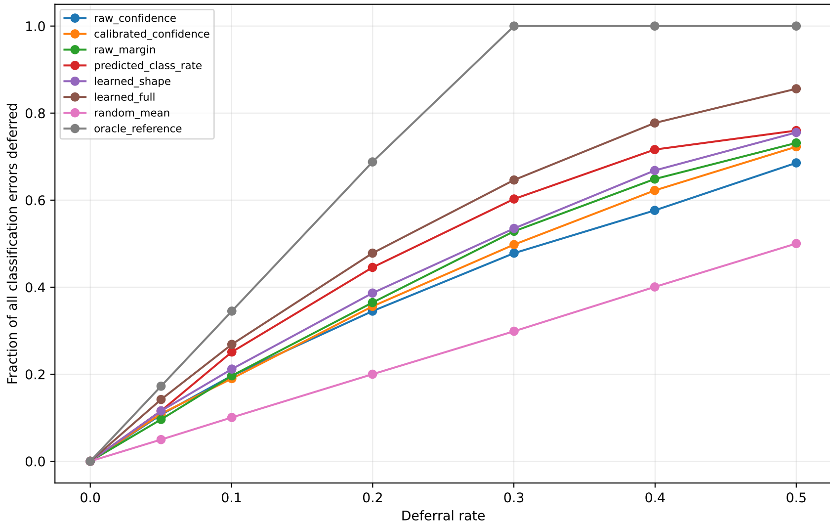
Error capture by ALerCE deferral policy
