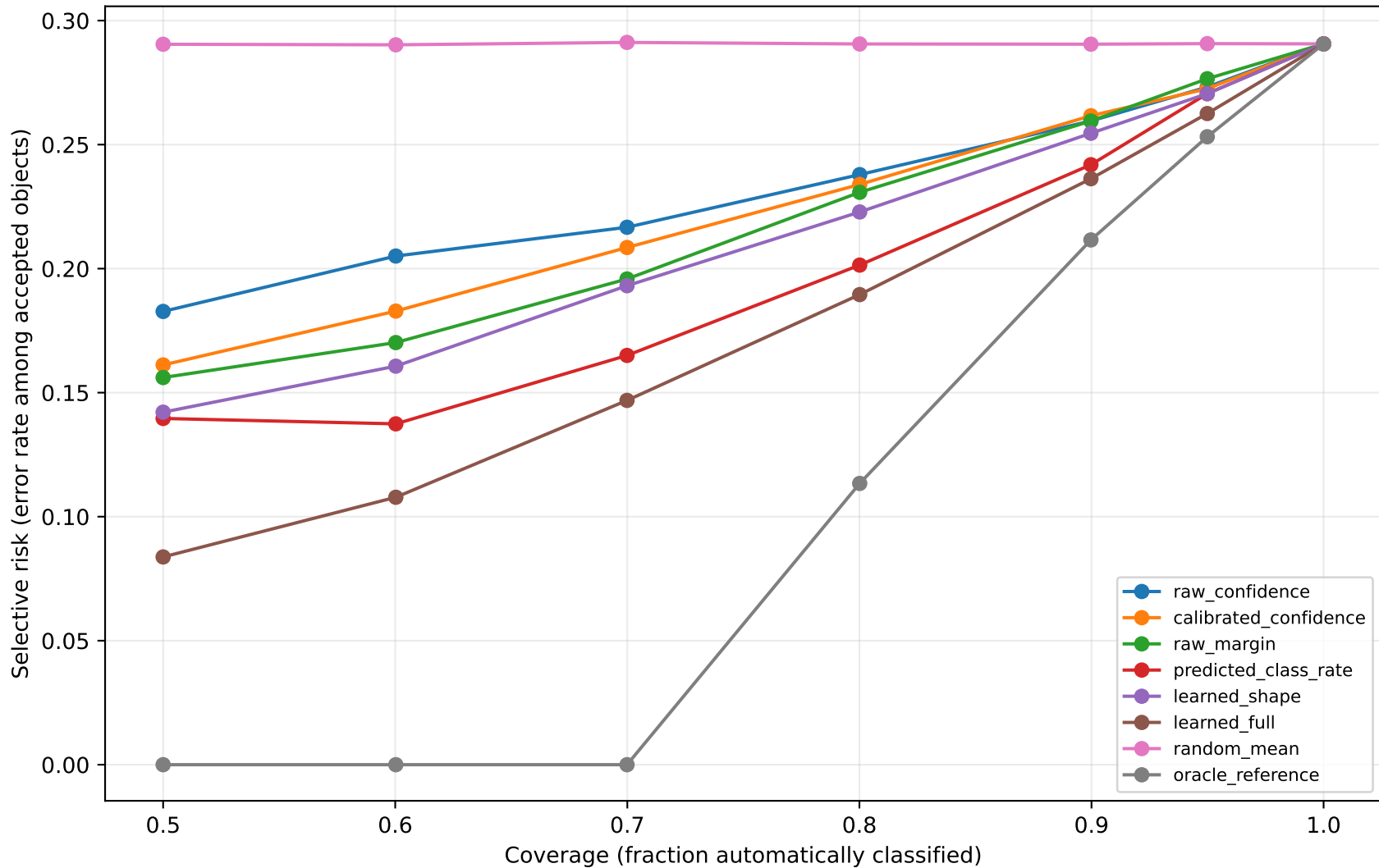
ALeRCE post-hoc deferral: risk-coverage comparison
