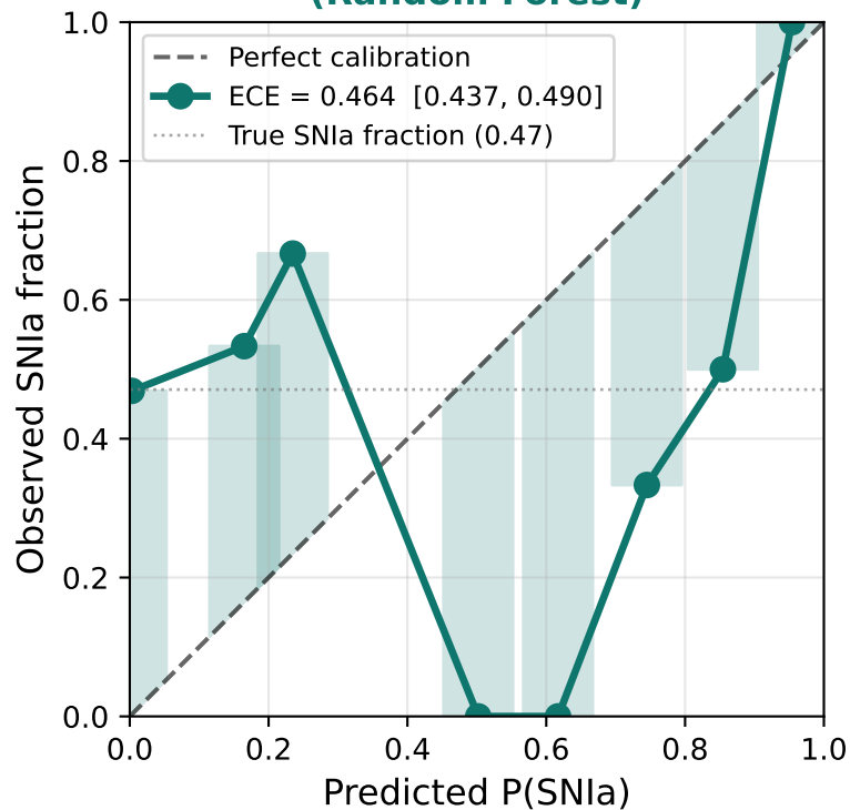
Fink — rf_sn1a_vs_non1a (Random Forest)
