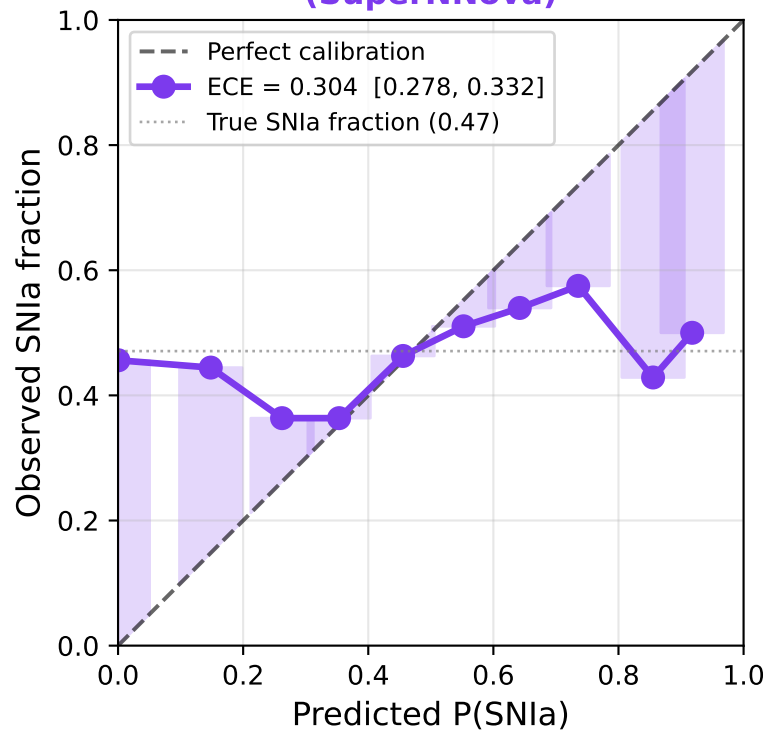
Fink — snn_sn1a_vs_non1a (SuperNNova)
