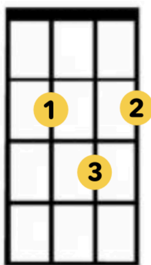
G major
