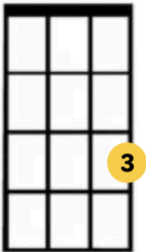
C major
