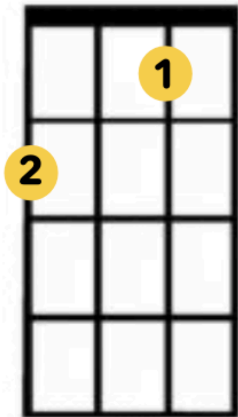
F major
