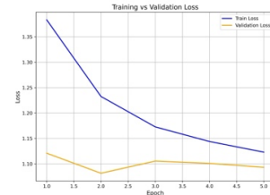
Figure 3: Modern BERT Losses Clean, Expansion=2.0, Dropout=0.25
