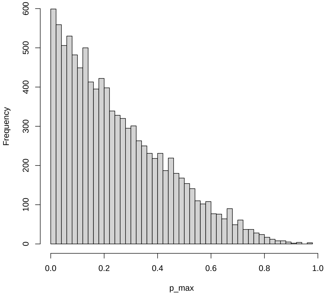
Distribution of maximum transmission probability
