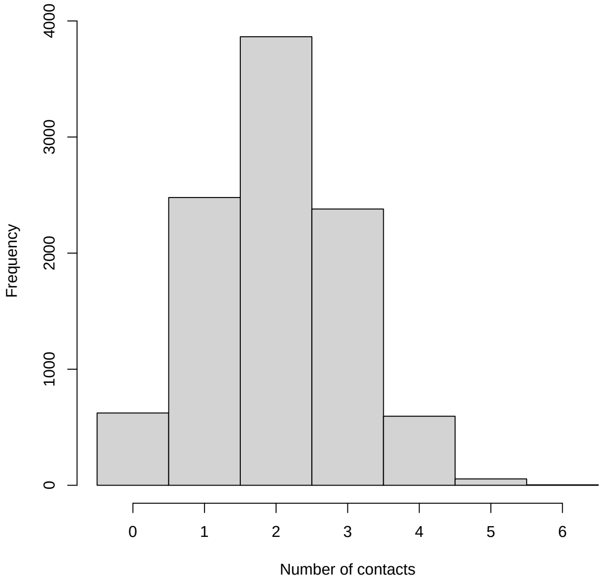
Distribution of nContact
