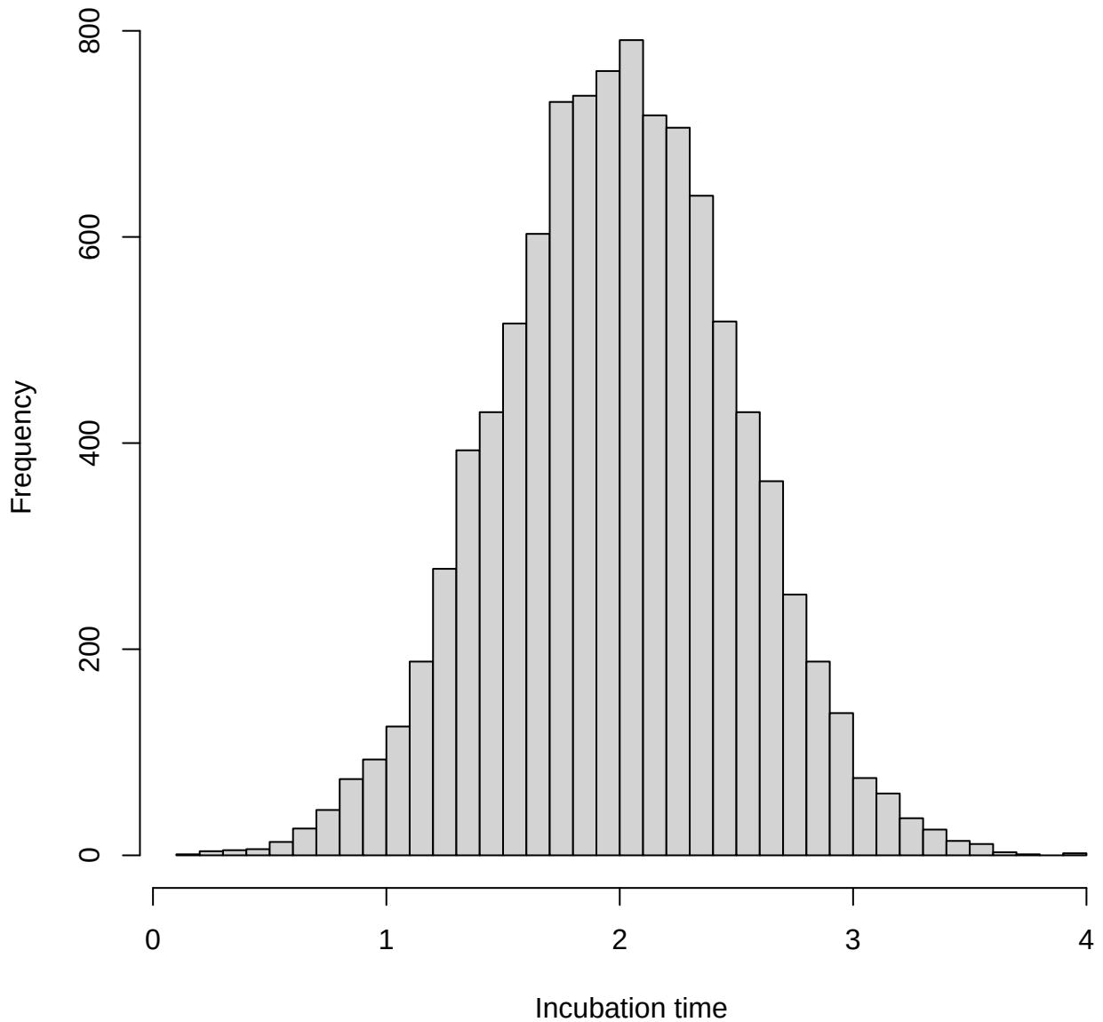
Distribution of incubation time
