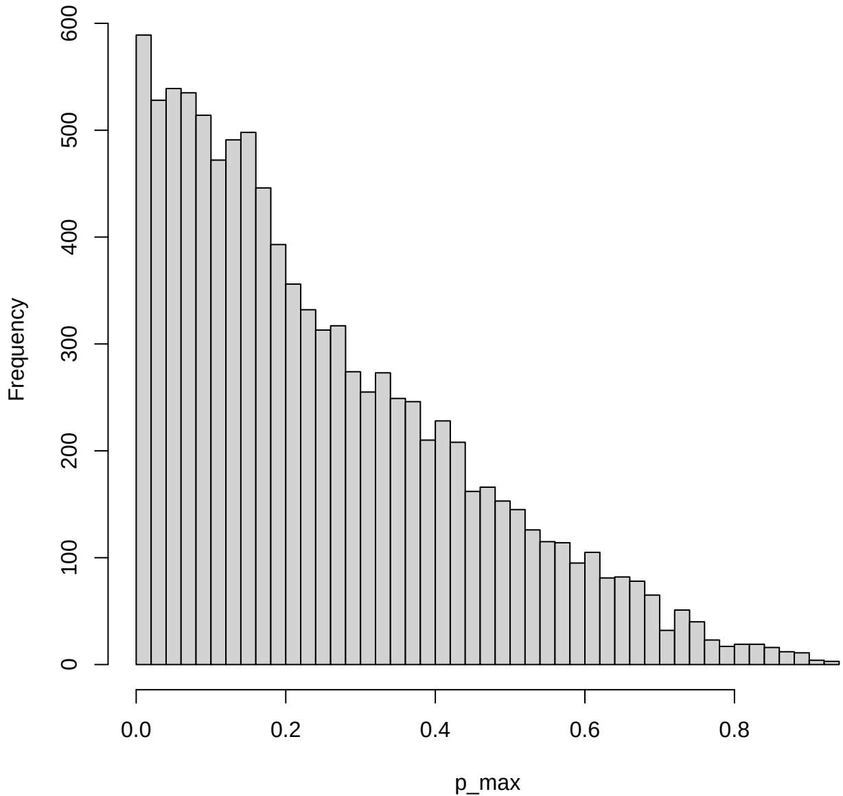
Distribution of maximum transmission probability
