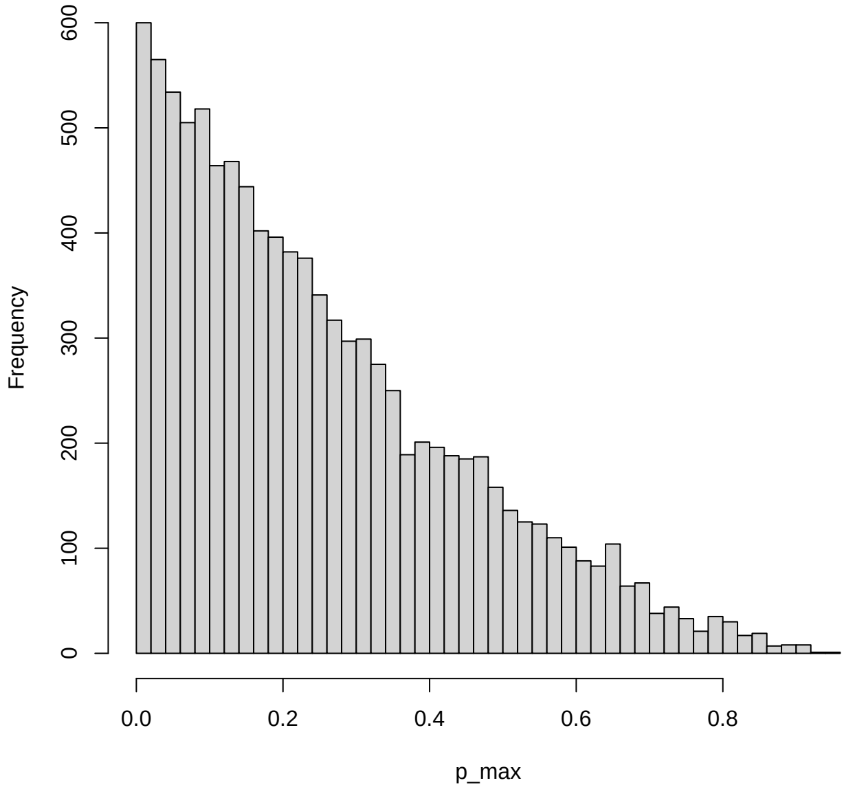
Distribution of maximum transmission probability
