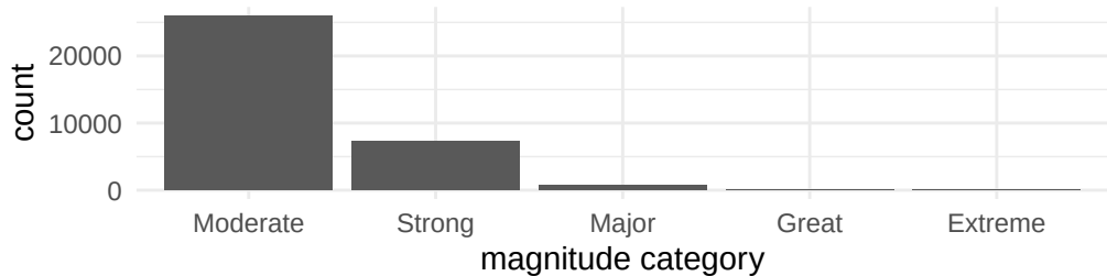
Distribution of Earthquake Magnitudes
