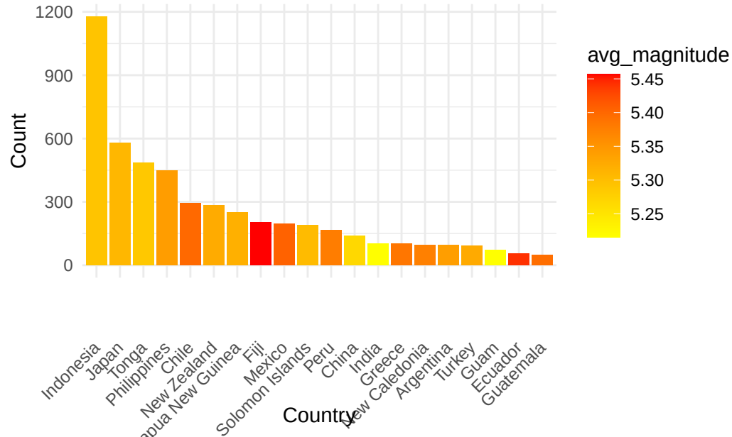
Top 20 Countries By Earthquake Count
