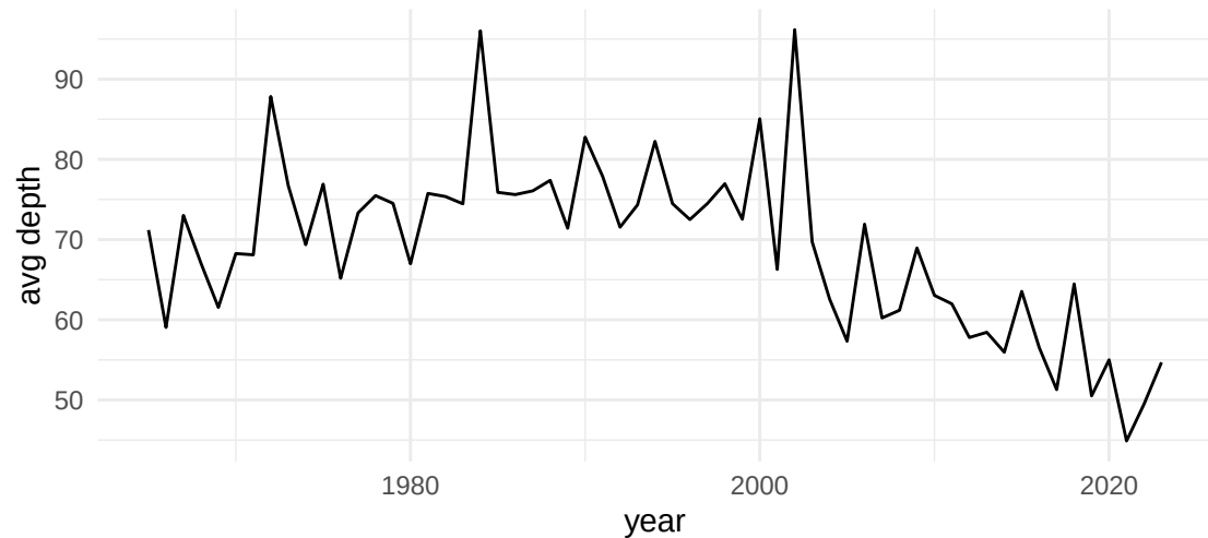
Yearly Average Earthquake Depth
