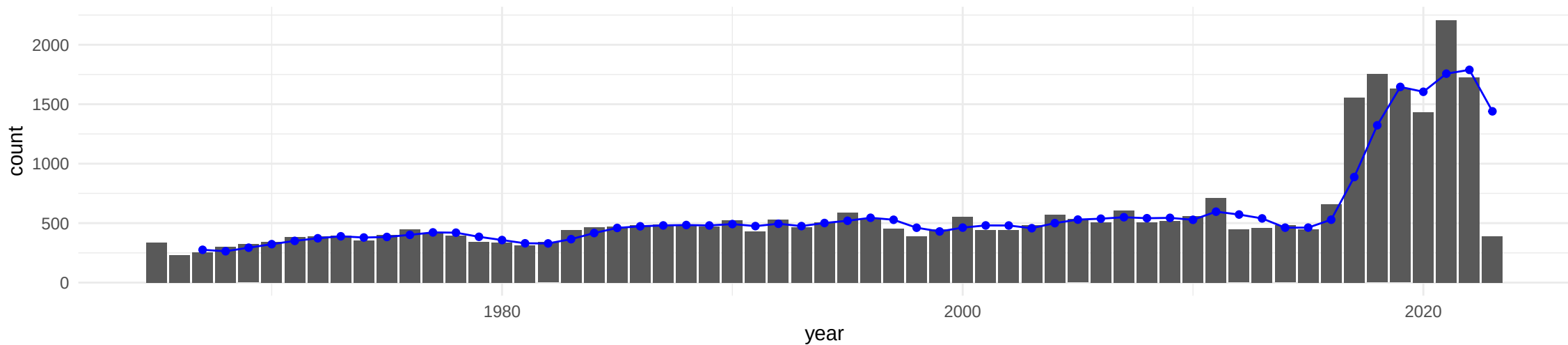
Number of Earthquakes per year
