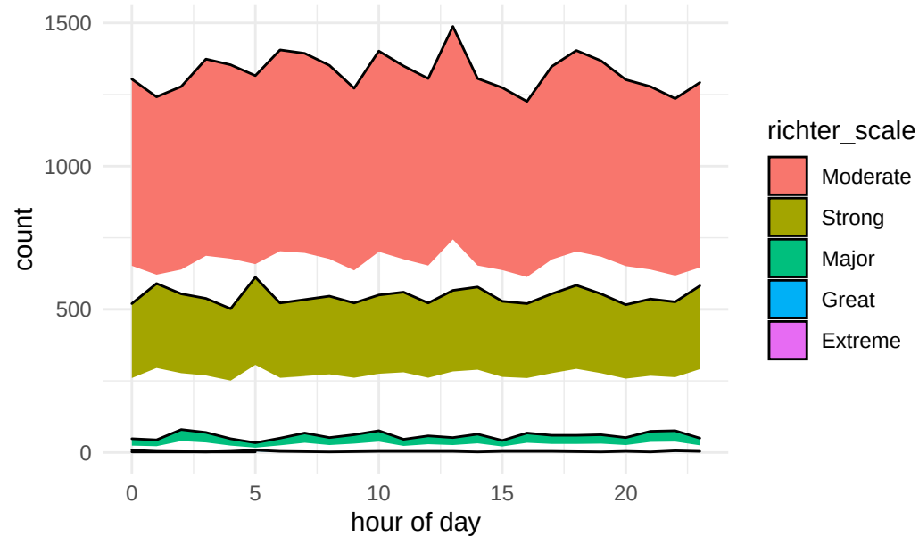
Hourly Count Earthquakes-Grouped by Category
