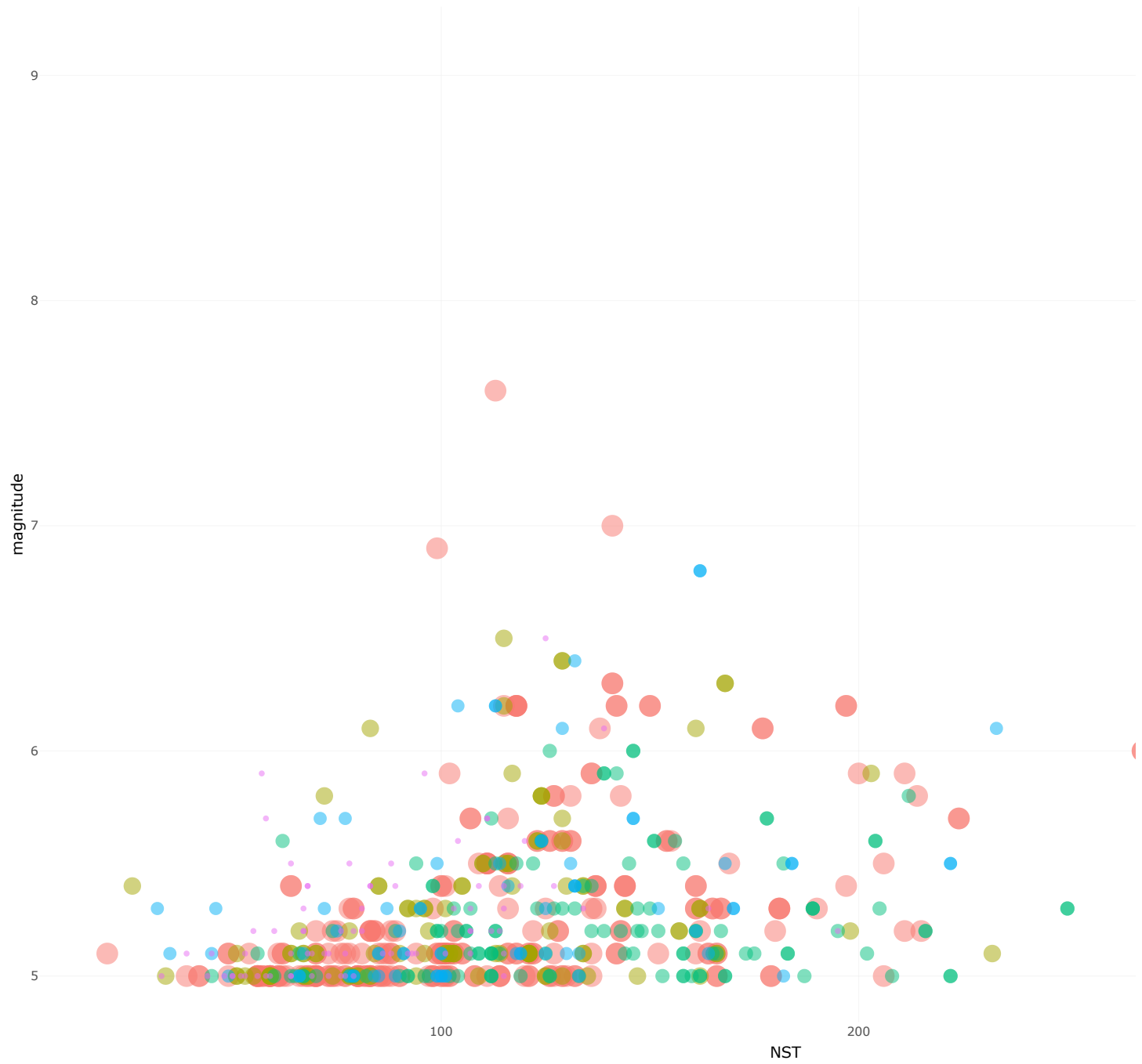
Avg Magnitude vs Avg Number of Siesmic Stations (NST)
