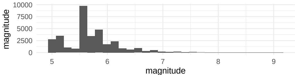
Distribution of Earthquake Magnitudes
