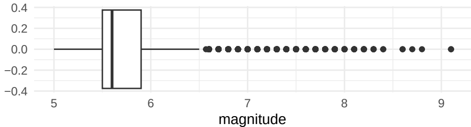
Distribution of Earthquake Magnitudes
