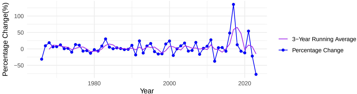
Yearly Percentage Change in Earthquake Count
