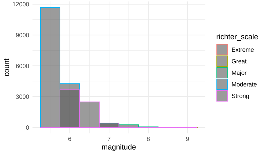
Earth Quake Magnitudes Per Richter Scale Category (All Ma
