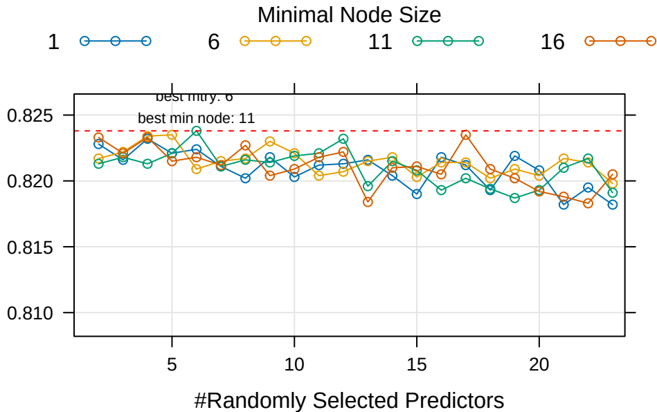
Accuracy Out of Bag Resampling
