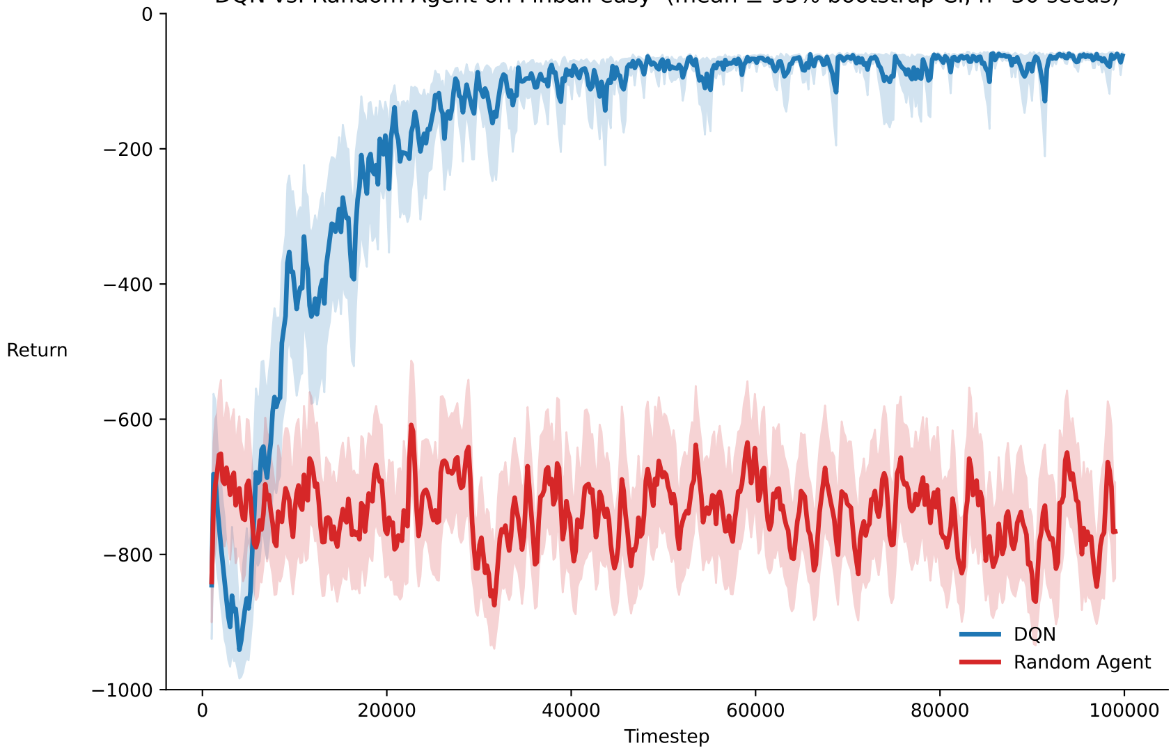
DQN vs. Random Agent on Pinball easy (mean \pm 95% bootstrap CI, n=30 seeds)
