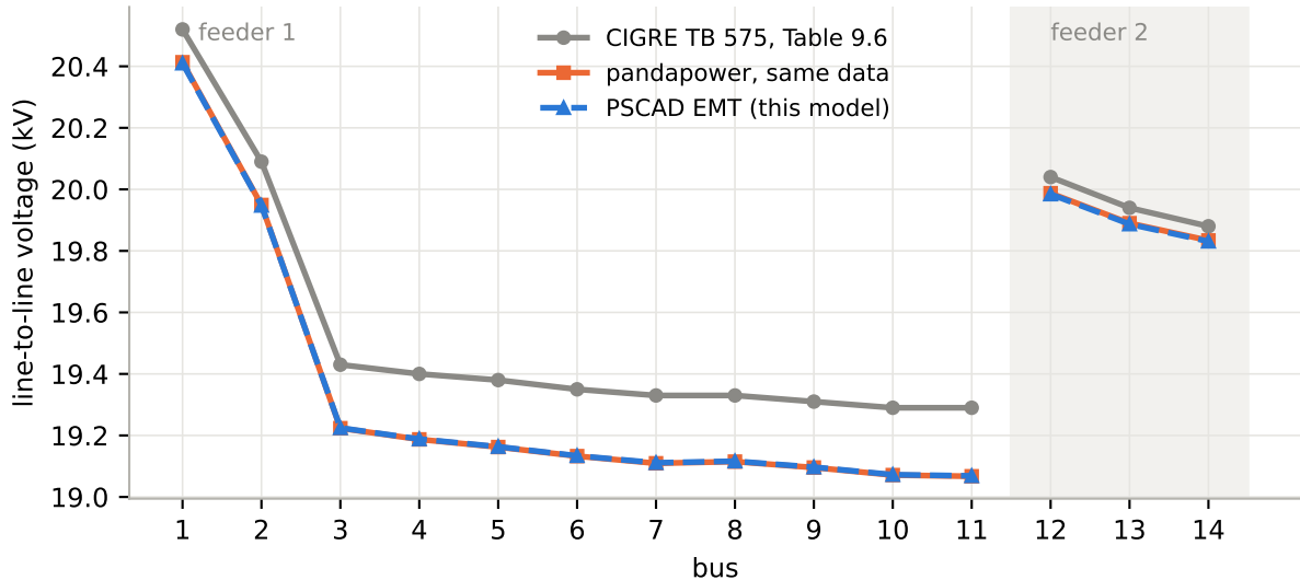
Steady-state voltage profile, radial base case
