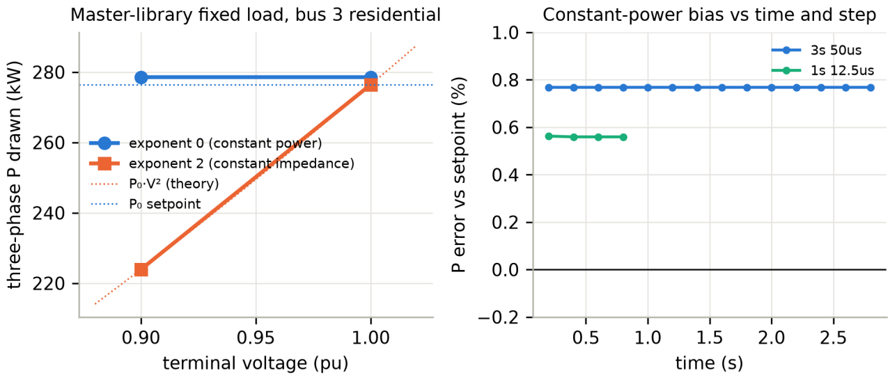
Figure 2. Master-library fixed load in a standalone test. Left: power drawn versus terminal voltage for exponent 0 and exponent 2, with the theoretical curves. Right: the constant-power bias versus time at two time steps.
