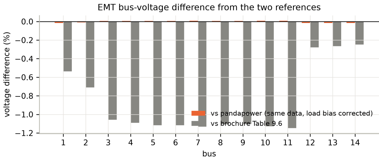
Figure 4. Difference of the EMT bus voltages from the two references.
