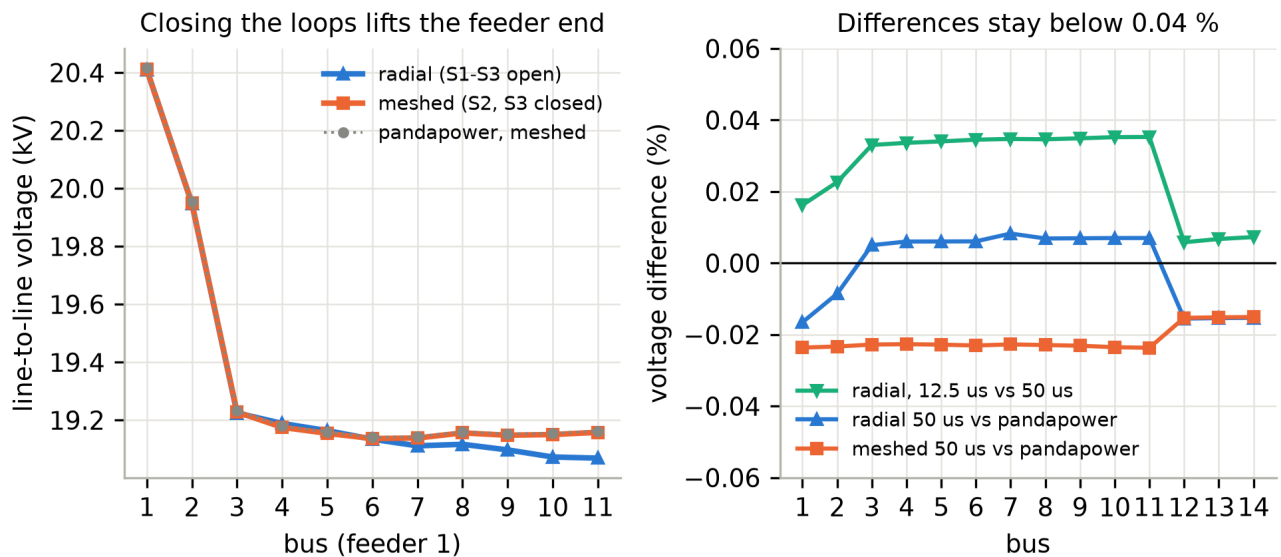
Figure 8. Left: feeder-1 voltage profile, radial and meshed, with the meshed load flow. Right: bus-voltage differences for the 12.5 \mu s run and for both configurations against the load flow.
