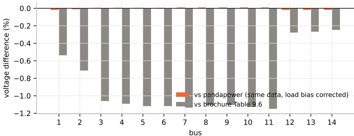
EMT bus-voltage difference from the two references
