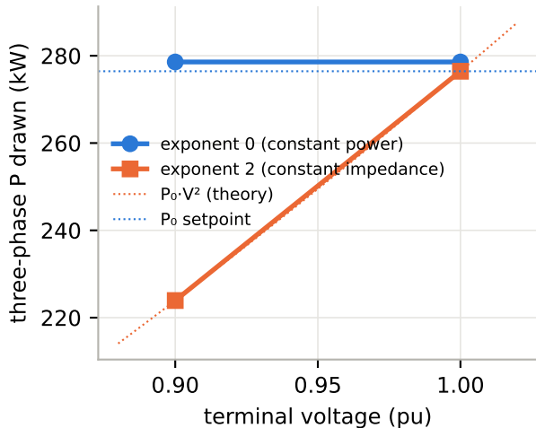
Master-library fixed load, bus 3 residential
