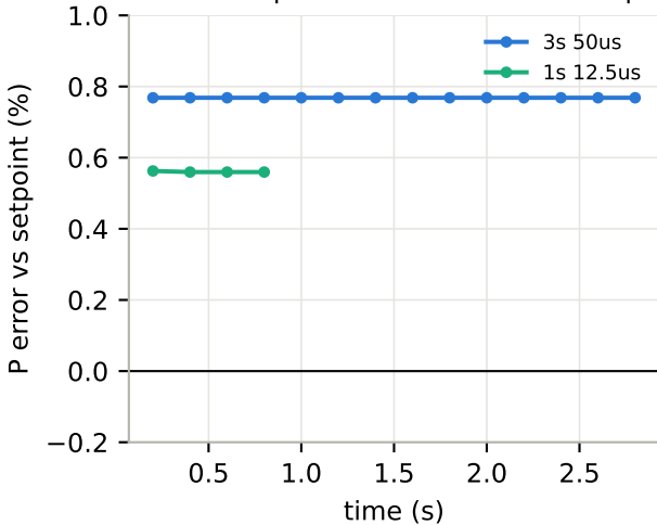
Constant-power bias vs time and step
