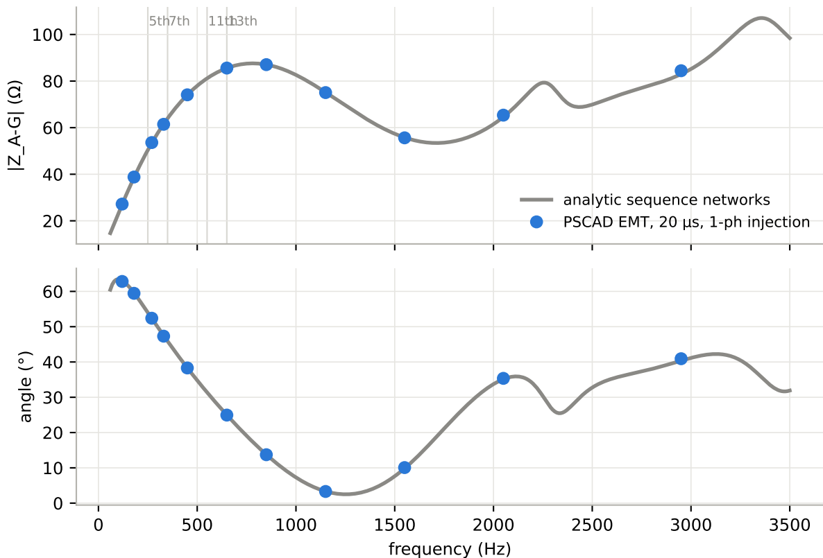
Phase-to-ground driving-point impedance at bus 11
