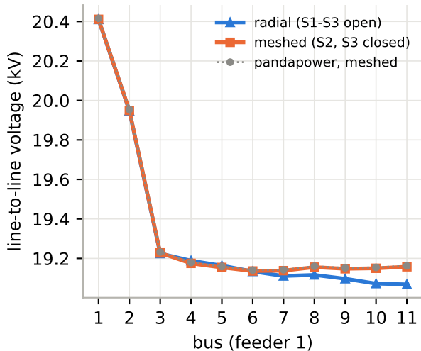
Closing the loops lifts the feeder end
