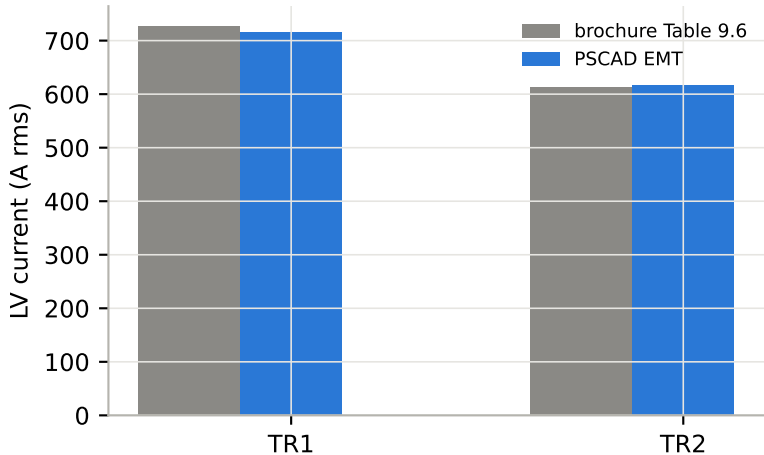
Transformer secondary currents
