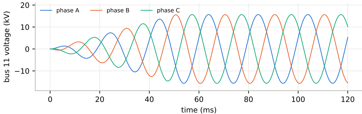
Base run start-up: 50 ms source ramp, then power settling
