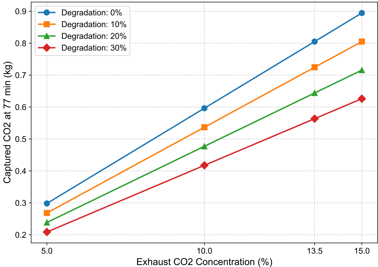
Sorbent Degradation vs. Exhaust Concentration
