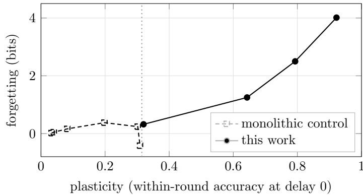
Figure 6: Each point is one learning rate, two or three seeds, Mode B at twelve regimes; the rate sweeps \eta \in \{0.1, \dots, 30\} for the control and \{0.1, \dots, 3\} for ours. The two arms do not overlap in plasticity at all: the control saturates at 0.309 and ours starts at 0.320, either side of the dotted line. Nothing about frontier position can be read from disjoint supports, which is why we report reachability only. Two features are worth stating rather than smoothing over: our forgetting grows steeply across our own range, 0.32 to 4.01 bits, so the high-plasticity end is not free; and the control’s highest-rate cell has negative forgetting, which we do not have an account for and treat as a sign that the control is unstable there rather than as a stability result.
