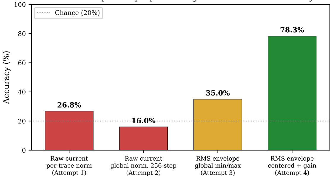
Ablation: Impact of preprocessing on classification accuracy
