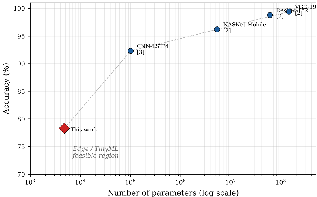
Accuracy vs. model size — broken rotor bar detection
