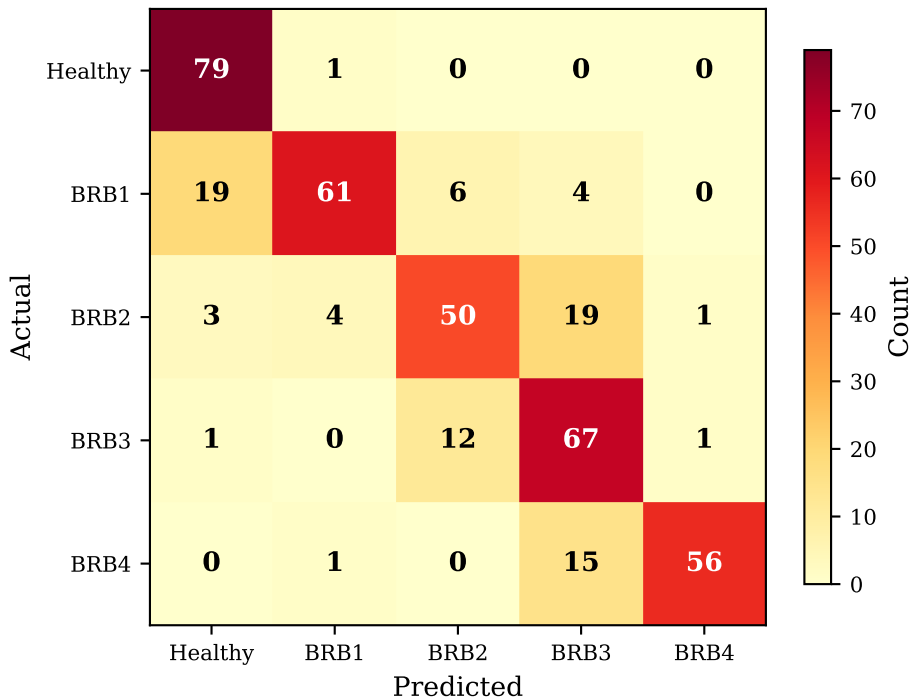
Confusion matrix — LSTM h=32, 80 epochs (78.3%)
