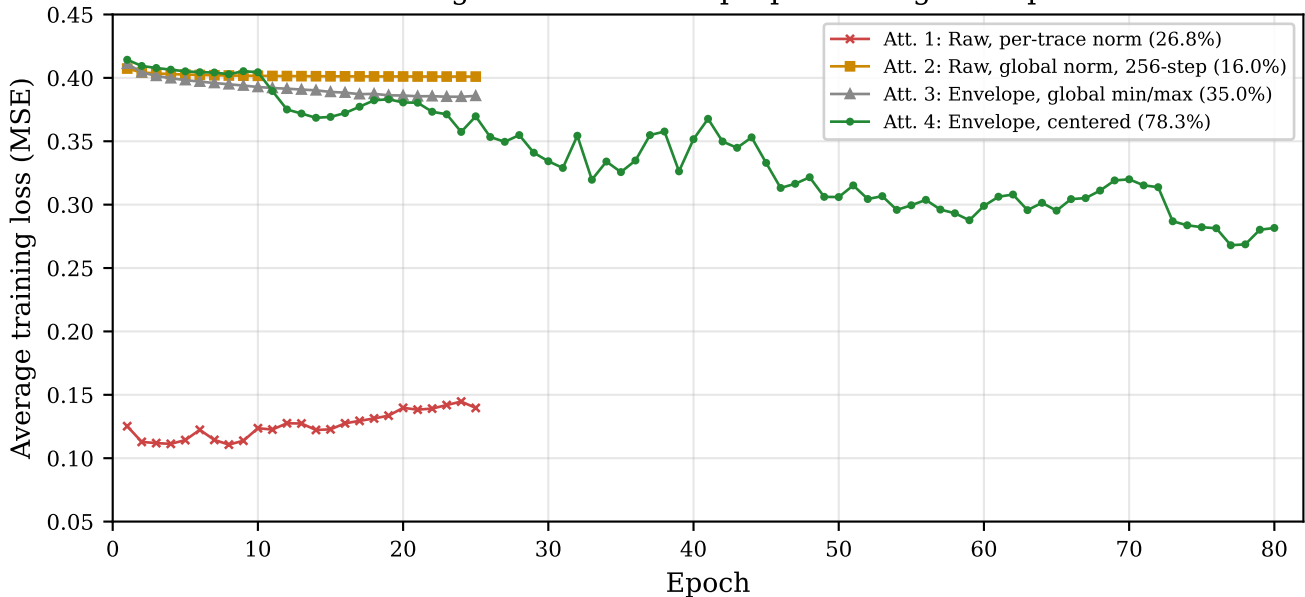
Training curves across 4 preprocessing attempts
