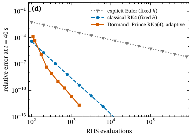
0D burn dynamics: work-precision
