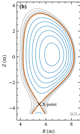
Solov'ev single-null (analytic)
