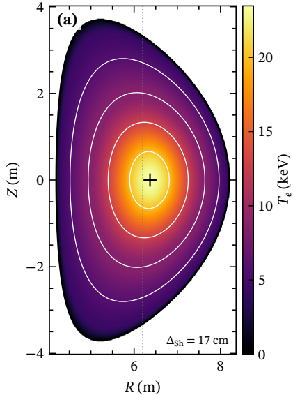
ITER 1.5D, t = 400 s
