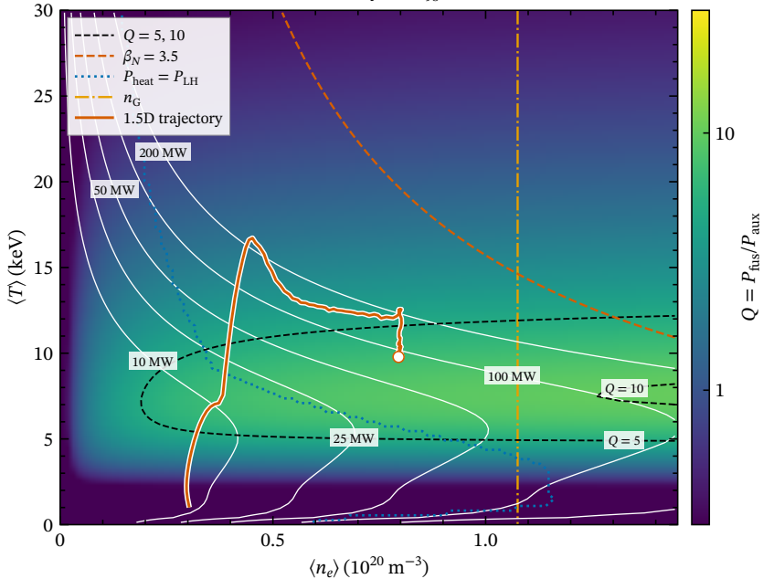
ITER (IPB98(y,2), H_{98} = 1 )
