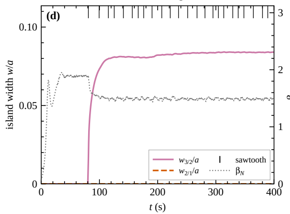
neoclassical tearing modes
