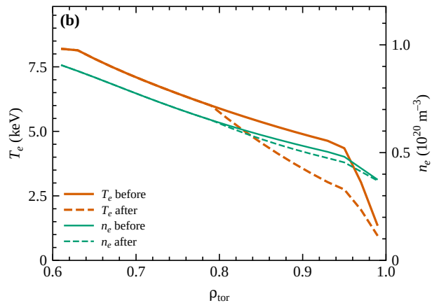
neoclassical tearing modes
