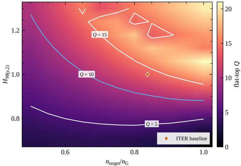
ITER 0D scan (11×11 runs)
