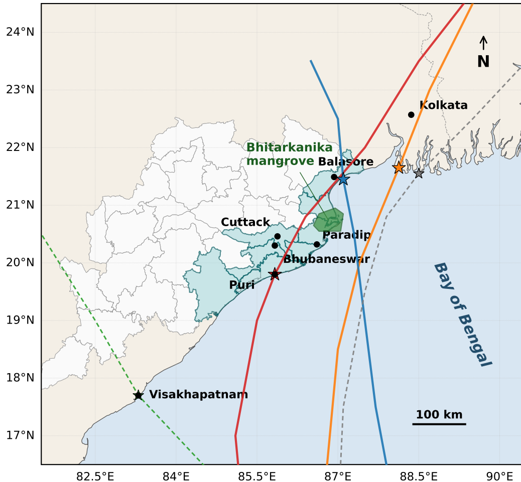
(b) Study area: 8 coastal-subcoastal districts of Odisha with cyclone tracks 2014–2021
