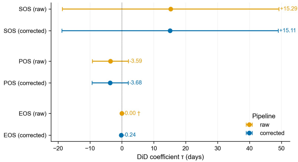
Figure 2. TWFE-DiD coefficients (raw vs. classifier-corrected panel). Point estimates with district-clustered (CR1) standard-error bars and 95% wild-cluster restricted bootstrap intervals for SOS, POS, and EOS, raw and corrected pipelines on the real v2.1 panel.
