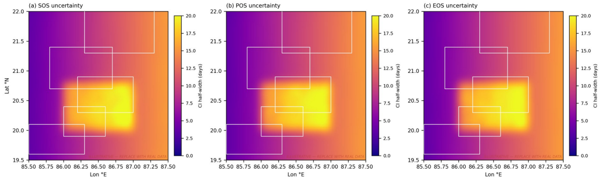
Figure 9. Pixel-level bootstrap 95% CI half-width for corrected SOS dates. Uncertainty highest in coastal shoreline pixels (cloud-gap-affected) and pixels with classifier marginal probability 0.4–0.6.
