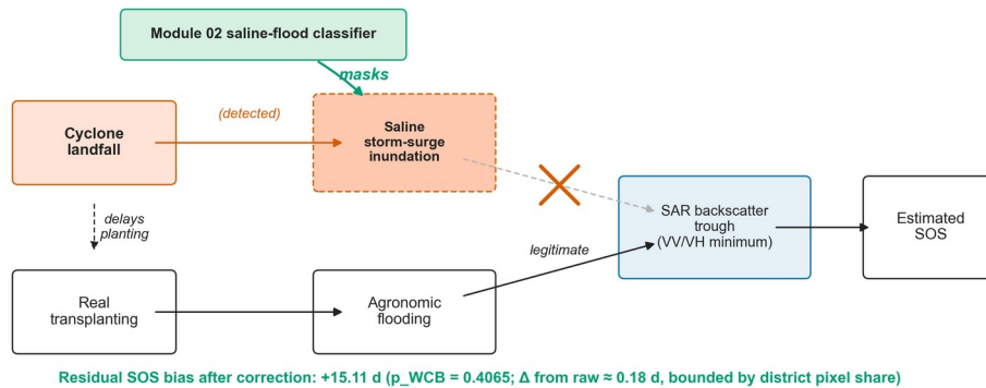
Figure 1B. Pearl-style identification DAG. Cyclone landfall ( T ) opens two pathways into the SAR backscatter trough: a legitimate transplanting-flood pathway and a confounding saline-surge pathway. Module 02 (the saline-flood classifier) intercepts the confounding pathway; the remaining backscatter trough identifies the agronomic SOS.
