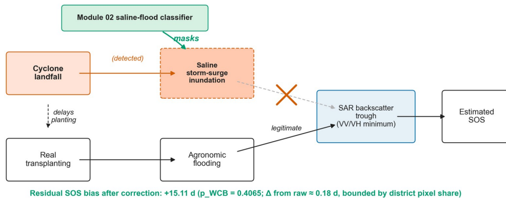
Figure 2. Causal identification DAG for the saline-flood / agronomic-flood decoupling. The cyclone landfall is a single exogenous shock that opens parallel legitimate (transplanting flooding) and confounding (saline storm-surge) pathways into the same SAR backscatter trough; the Module 02 saline-flood classifier intercepts the confounding pathway.
